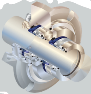
ISC2 Double Seal
