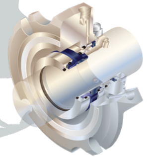
ISC2 Single Seal
