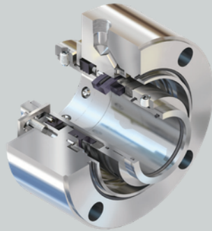
BX Single Seal
