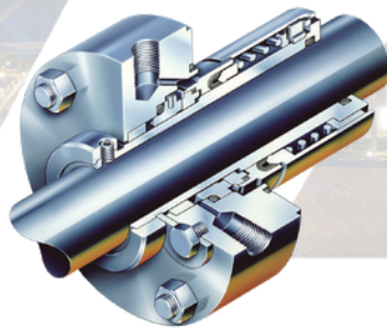
UC Pusher Seal
